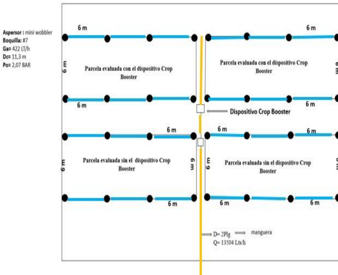
Figure 2: Hydraulic design of the irrigation system
